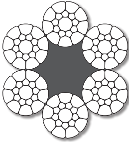
6x19 Compacted
