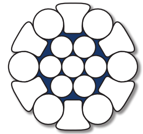
Half Lock Guide Rope
