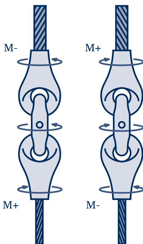
Fig. 59: Connection of wire ropes with equal direction of lay but different diameters
