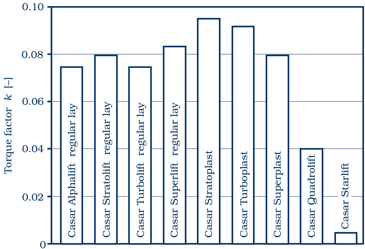
Fig. 9: Torque factor k for different Casar special wire ropes
