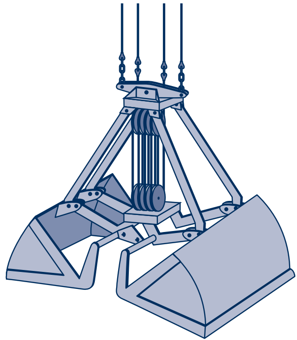
Fig. 56: Four-rope grab with two holding and two closing ropes
