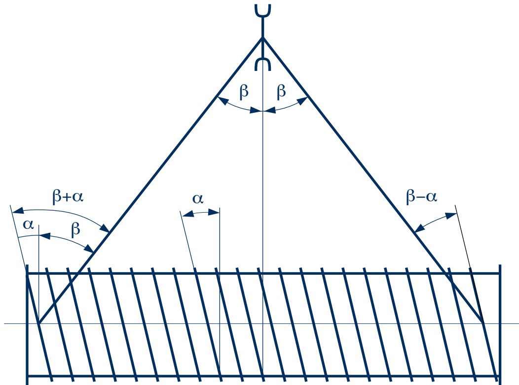
Fig. 37: Fleet angles at the drum and the sheave
