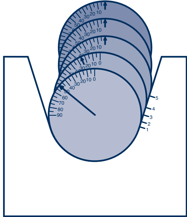
Fig. 35: Great twist of a rope when the fleet angle is 5°
