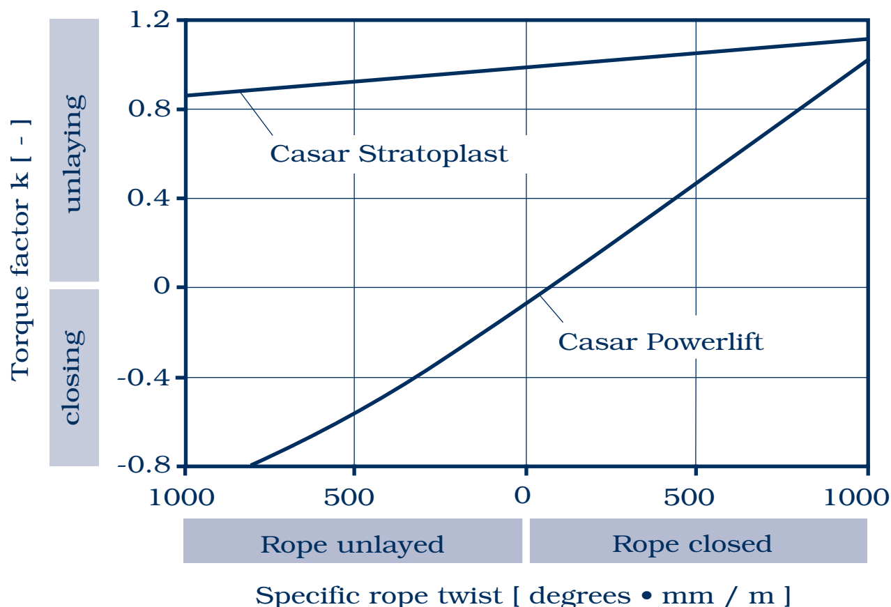
Fig. 28: When, for instance, rotation is enforced by slewing the crane, rotation-resistant ropes develop much greater counteracting moments than non-rotation-resistant ropes.
