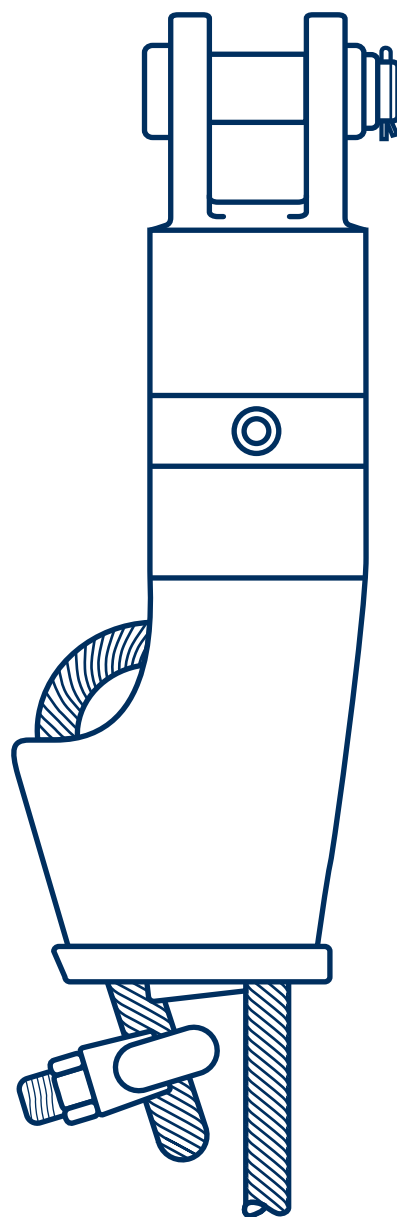
Fig. 54: Wedge socket with a built-in swivel
