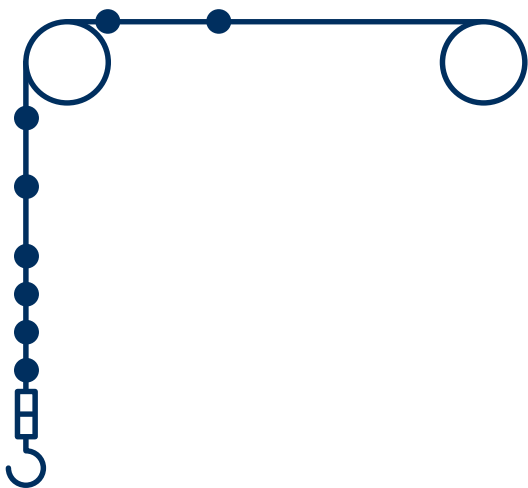
Fig. 47: Part of the twisted rope length runs back over the sheave.
