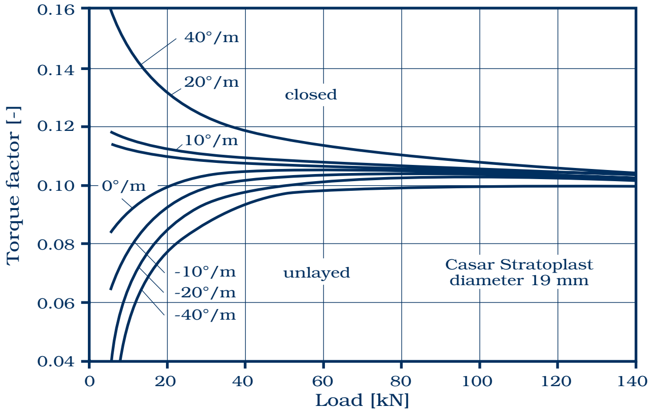
Fig. 31: The changes of the torque factor of a non-rotation-resistant wire rope caused by enforced rotation. The factor k is hardly changed.
