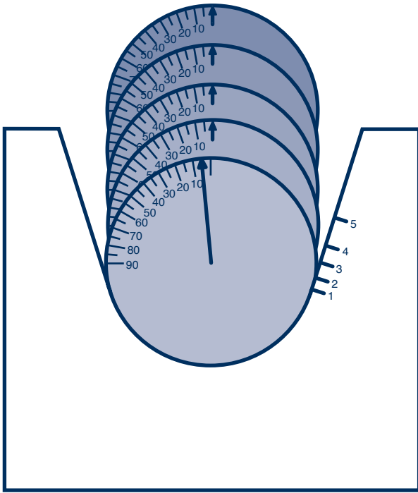
Fig. 34: Slight twist of a rope when the fleet angle is 1°
