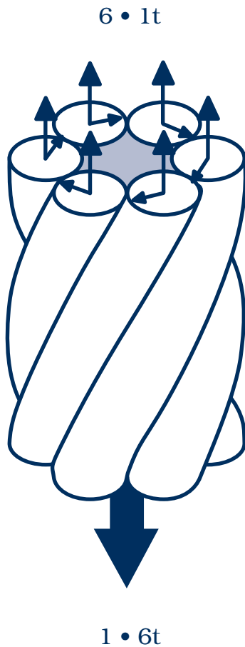
Fig. 3: Closed wire rope
