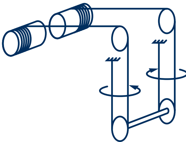
Fig. 25: Crane with left-hand lay and right-hand lay wire ropes
