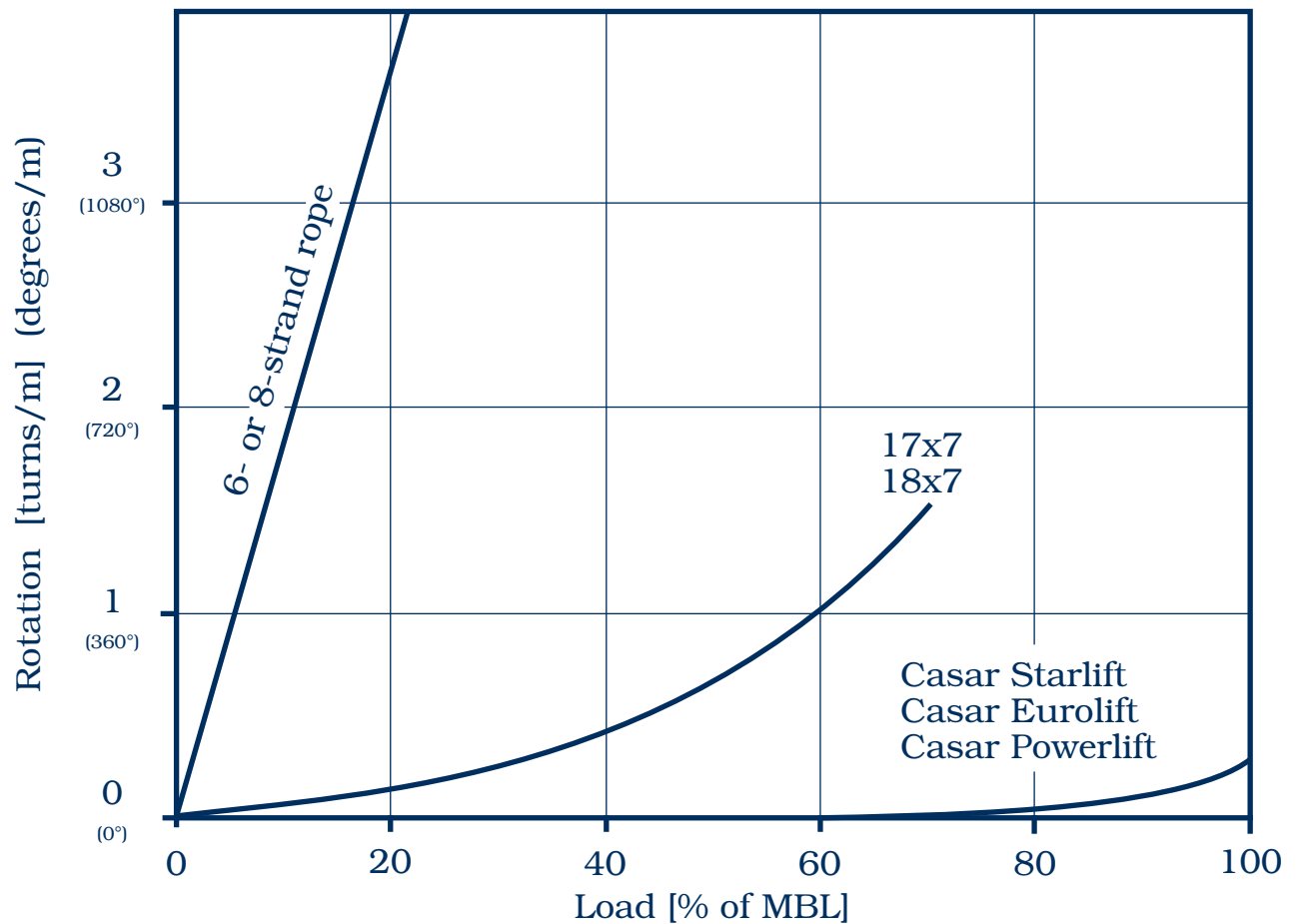
Fig. 15: Angular rotation of different rope constructions in a break test with an open swivel
