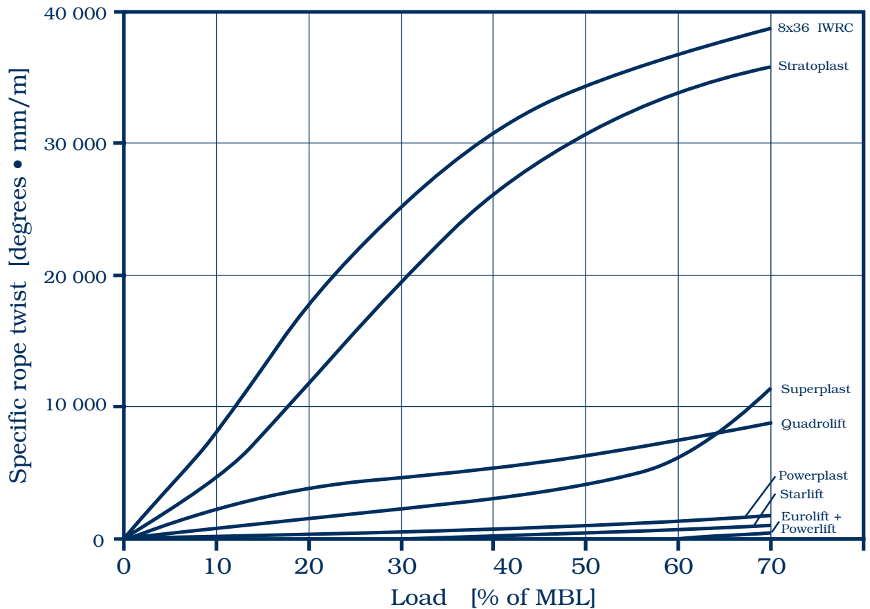
Fig. 10: Angular rotation of different wire rope designs when under load
