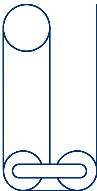
Fig. 24: A comparatively unstable three-part reeving
