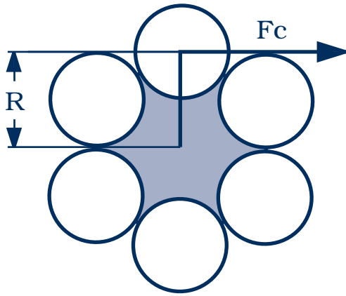
Fig. 6: The moment of the wire rope
