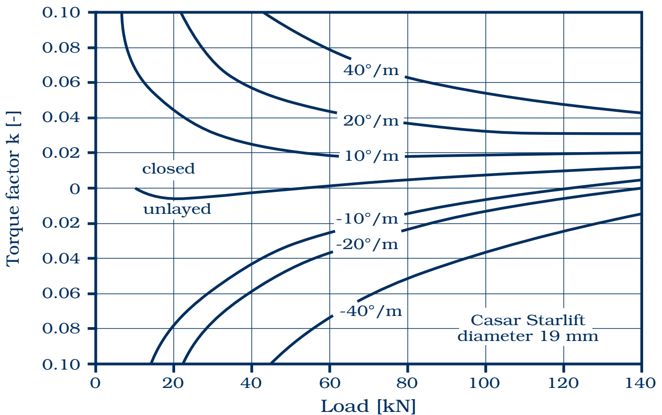
Fig. 32: The changes of the torque factor of a rotation-resistant rope, caused by enforced rotation. The factor k is changed considerably.
