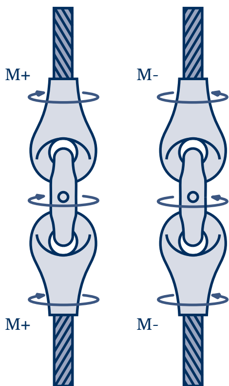
Fig. 58: Incorrect connection of grab ropes. The ropes unlay each other.
