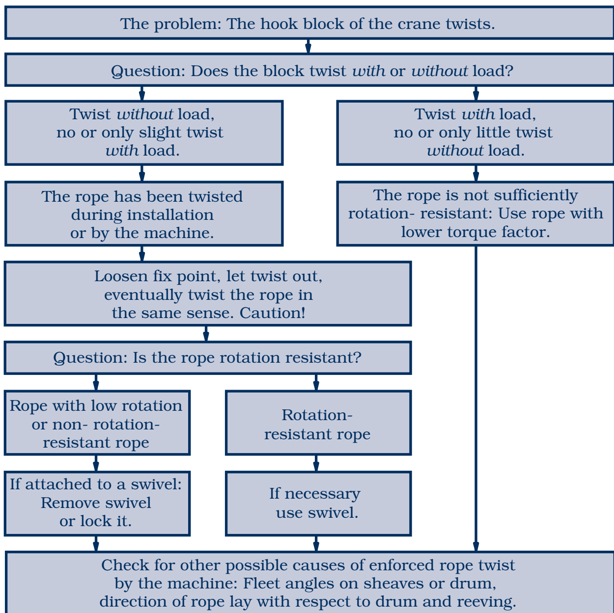
Fig. 55: First aid - What to do in the event of a rotating hook block.
