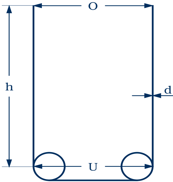
Fig. 21: Dimensioning the reeving
