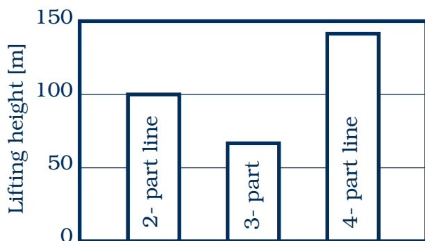
Fig. 23: The influence of the number of parts on the maximum permissible lifting height
