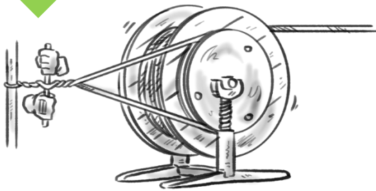
Application of the preload using a braking disc at the reel
