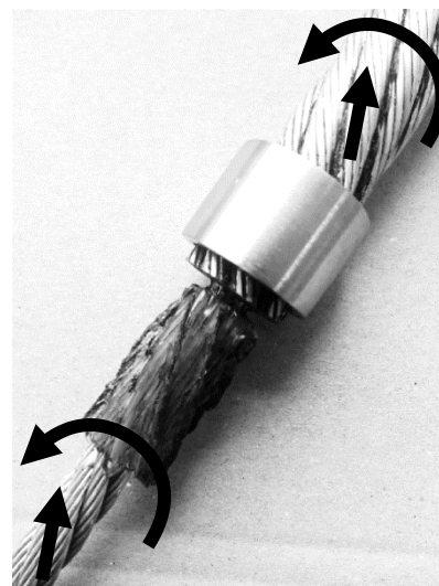
Non-rotation-resistant
